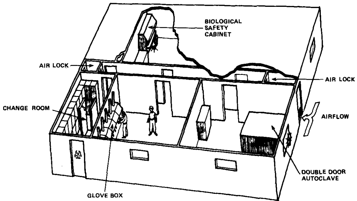
SECONDARY BARRIERS IN REPRESENTATIVE P4 FACILITY
