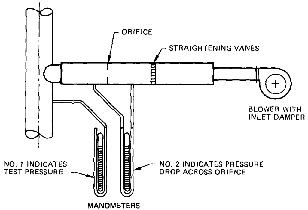
MANOMETERS USED FOR LEAK TIGHTNESS TESTING
